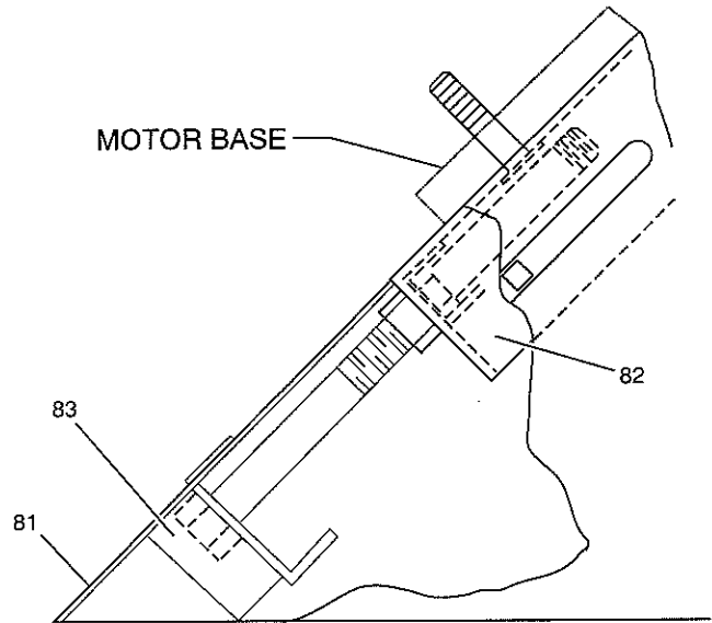
MOTOR MOUNTING / BELT TENSIONING ASSEMBLY FIG. 4
