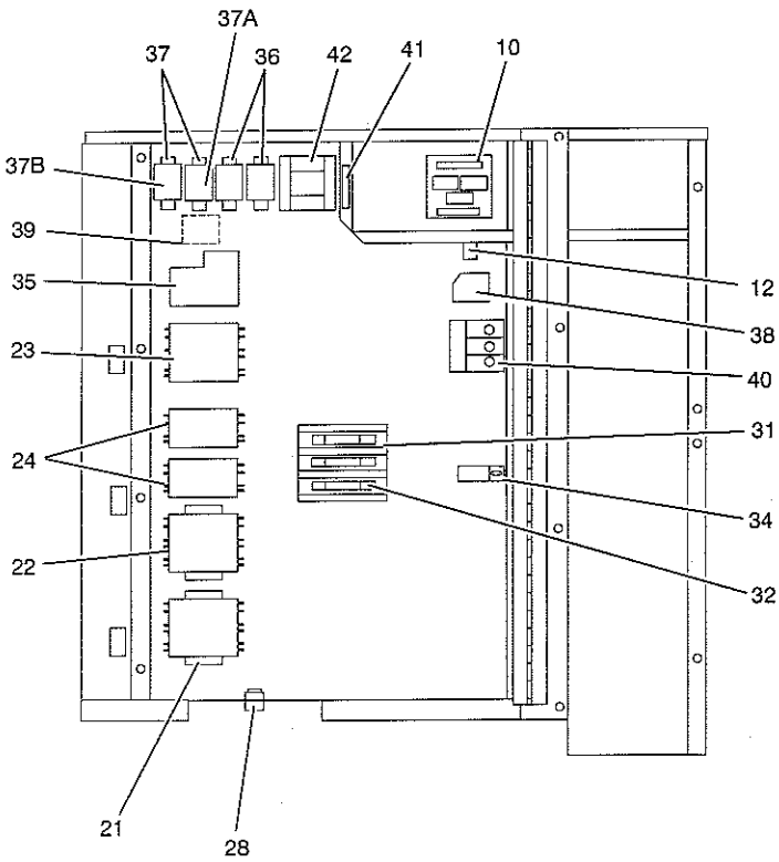
FIG. 3 - ELECTRICAL BOX
